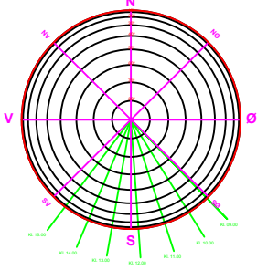
Solens bane 21. december
